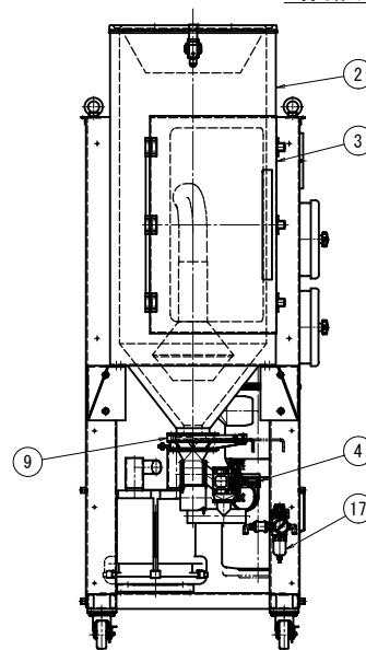
A arrow view A矢視
